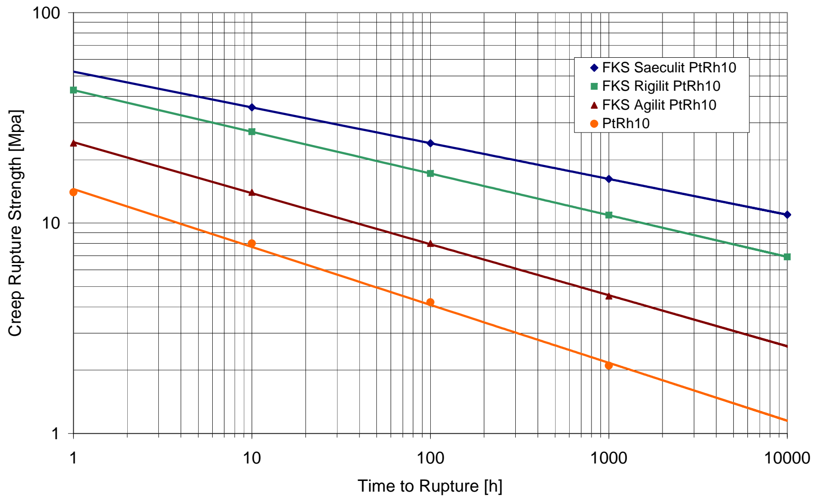
Creep Rupture Strength vs. Time to Rupture (1400°C)
