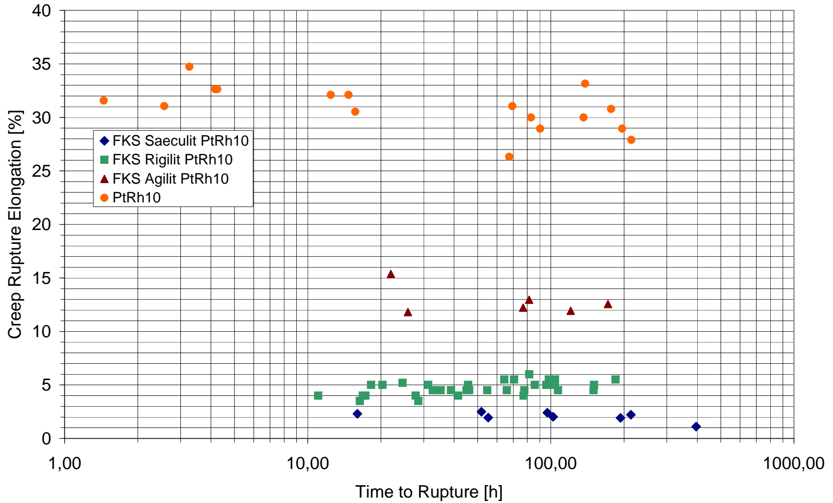
Creep Rupture Elongation vs. Time to Rupture (1400°C)
